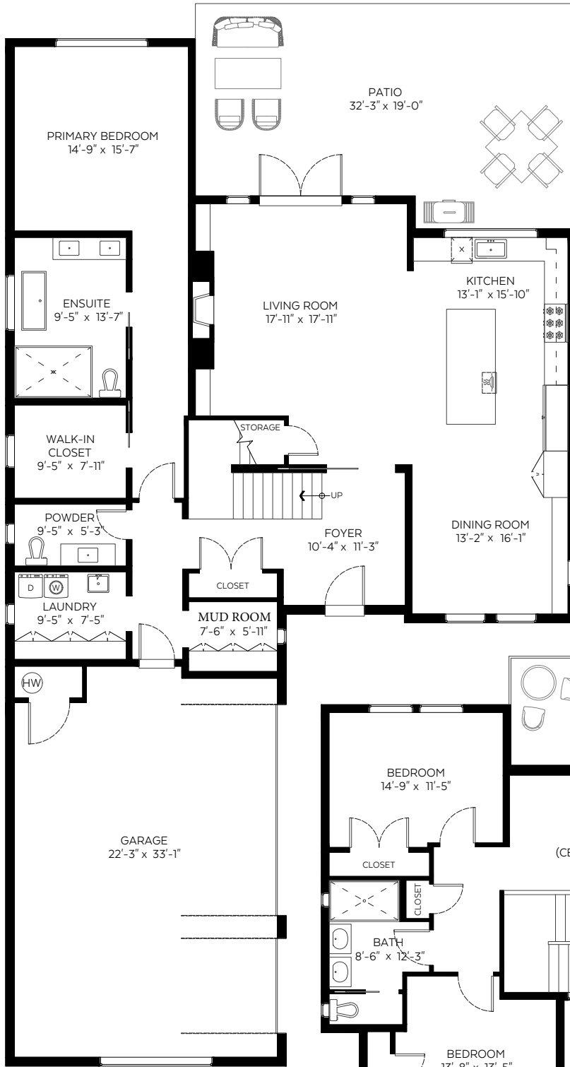
Main Floor Plan Floor Area: 2,013 sq.ft. Ceiling Height: 10 ft.
