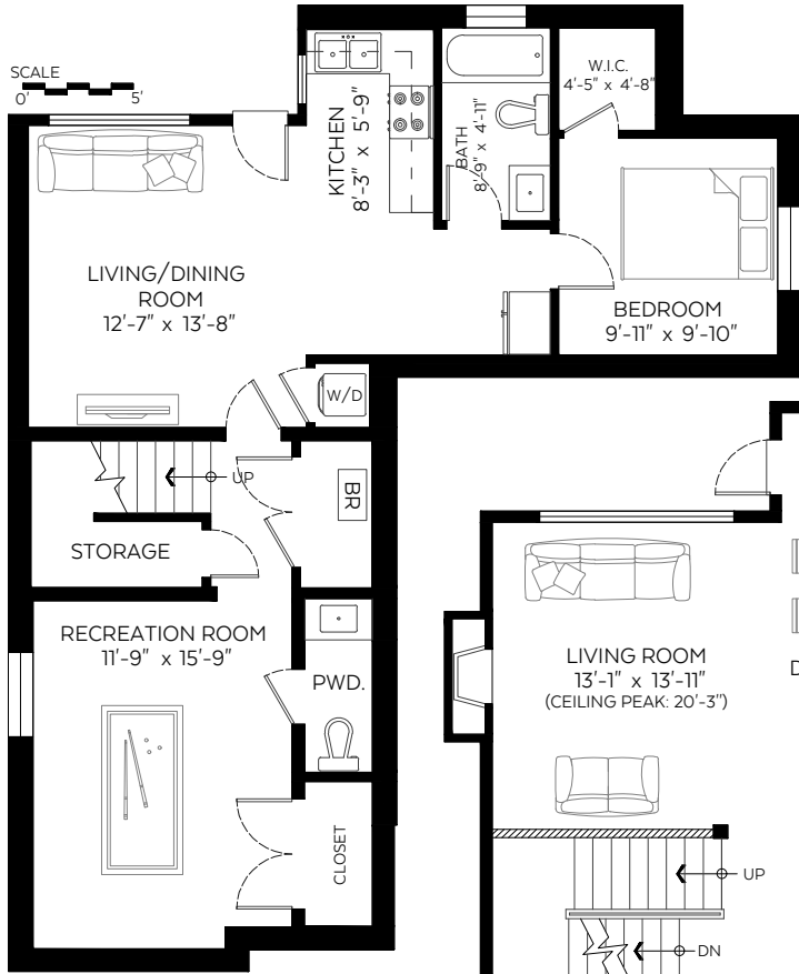
Lower Floor Plan Floor Area: 982 sq.ft. Ceiling Height: 8 ft.
